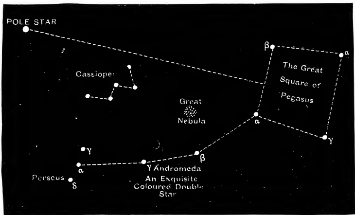
Fig. 91.—The Great Square of Pegasus.
